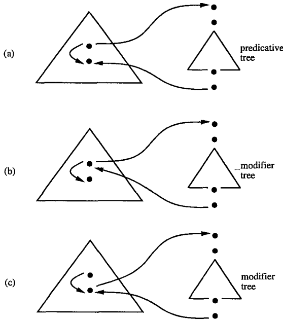
Figure 8 Schematic structure of possible predicative and modifier adjunctions with top and bottom of each node separated.
