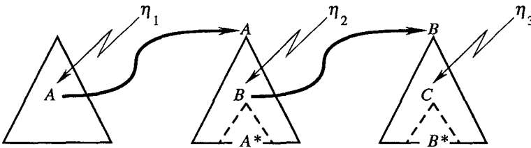
Figure 7 A stack of indices [\eta_1 \eta_2 \eta_3] captures the adjunction history that led to the reaching of the node \eta_3 in the parsing process.
