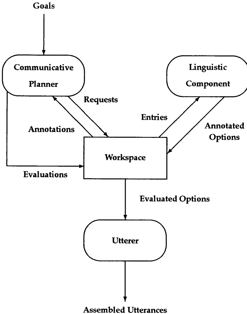
Figure 2 Architecture of the IGEN generator.
