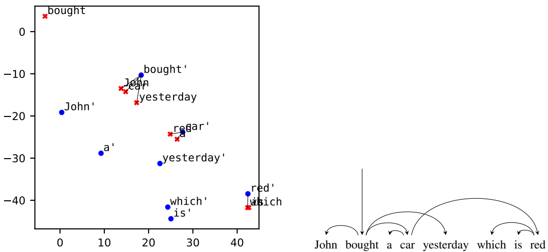
Figure 9: A sentence with a non-projective dependency structure: John bought a car yesterday which is red
