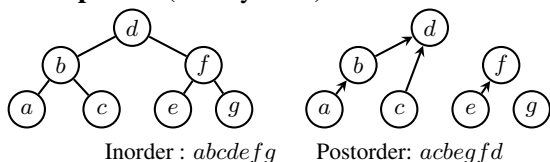
Figure 2: An example binary tree and a partial order over the vertices induced by two total orders. ■
