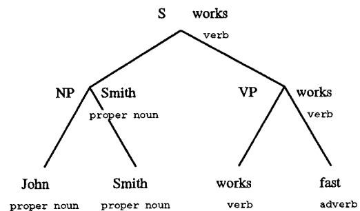
Figure 1: Sentence with Parse Tree and Headwords
