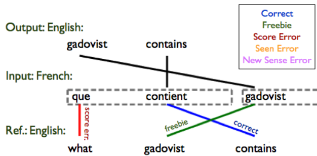
FIGURE 1: Example of WADE visualization. Dashed boxes around the French input mark the phrase spans used by the decoder.
