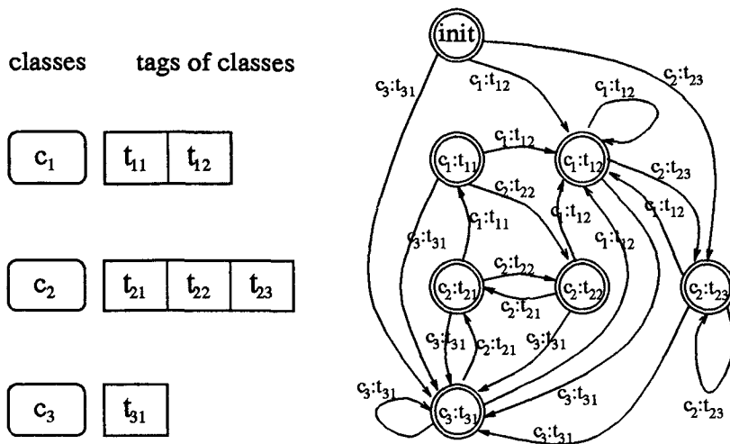
Figure 1: Generation of an n1-type transducer
