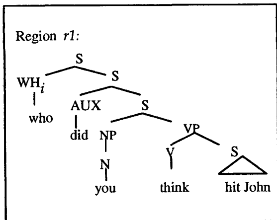
Figure 5: Final tree: Who did you think hit John?
