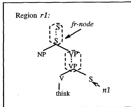
Figure 2. Initial tree selected in region r_1
