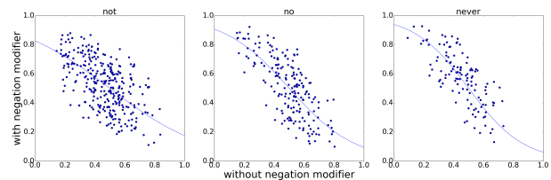
Figure 2: The sentiment shifts with negators. Each dot \langle x, y \rangle indicates that x is the sentiment score of a phrase without negator and y is that of the phrase with a negator.
