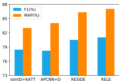
Figure 4: Comparison on GIDS-FB8K dataset.
