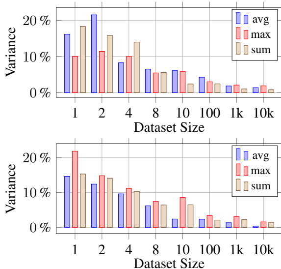
Figure 7: Sample variance across different subset sizes on the RST-DT dataset (top) and Instr-DT corpus (bottom)
