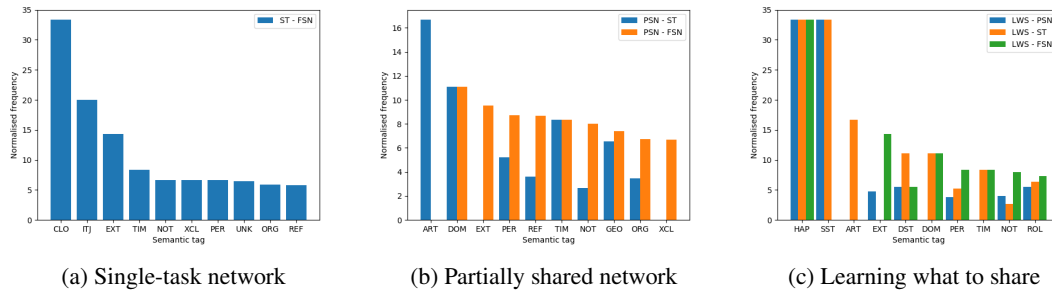
Figure 2: Normalized semantic tag frequencies for all six sets of sentences. X - Y denotes the set of sentences correctly classified by model X but misclassified by model Y .
