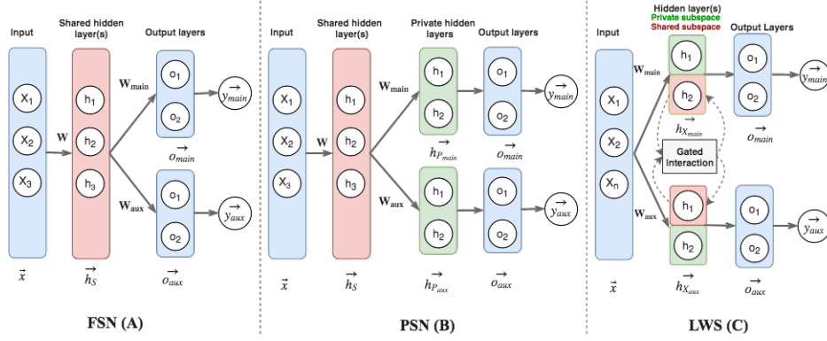
Figure 1: Our three multi-task learning settings: (A) fully shared networks, (B) partially shared networks, and (C) Learning What to Share . Layers are mathematically denoted by vectors and the connections between them, represented by arrows, are mathematically denoted by matrices of weights. S indicates a shared layer, P a private layer, and X a layer with shared and private subspaces.
