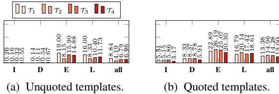
Figure 4: Prompt-based performance of mBERT, using alternative German templates.
