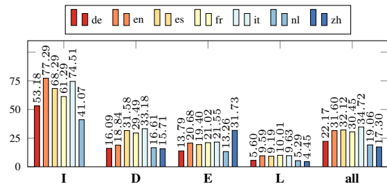
(a) fastText models from Grave et al. (2018).
