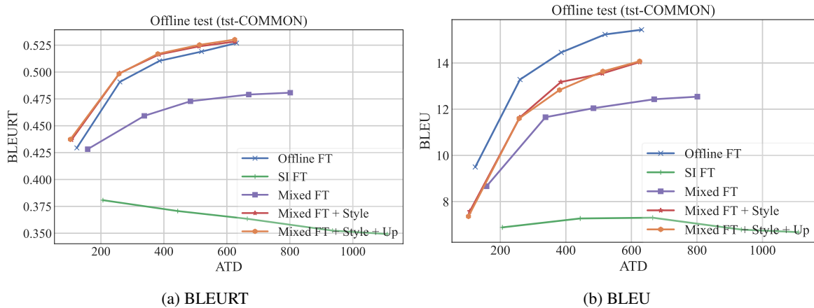
Figure 3: SimulST latency (ATD) – quality results on offline test set.
