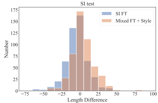
Figure 6: The length differences between hypotheses and references in SI FT and Mixed FT + Style (speech segment size is 600ms) on SI test set.
