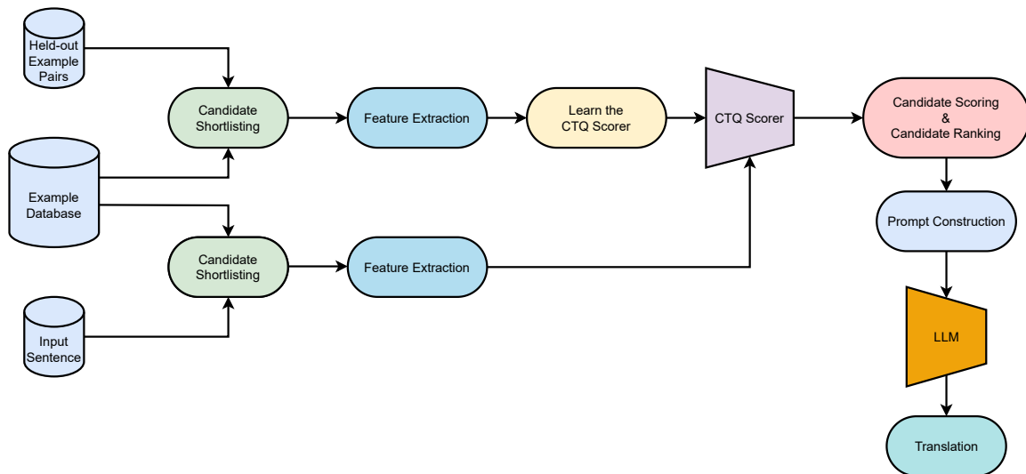
Figure 1: Overview of our LLM-based example selection system. The system selects in-context examples by incorporating multiple features to estimate the Contextual Translation Quality (CTQ) score. The upper part of the figure illustrates the training process of the CTQ Scorer. Candidate shortlisting is conducted using held-out example pairs, and feature extraction is performed on these shortlisted candidates. The extracted features are used for the training of the CTQ Scorer. During the inference stage, as depicted in the lower part of the figure, candidate shortlisting is performed for an input sentence from the examples in the example database, and relevant features are extracted. The CTQ Scorer then performs candidate scoring and ranking based on these extracted features. Subsequently, the best examples are chosen based on the CTQ score, and a prompt is constructed. Finally, the LLM produces the machine translation output using this constructed prompt.
