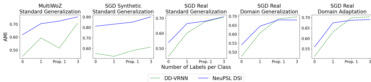
Figure 3: Average AMI for MultiWoZ, SGD Synthetic, and SGD Real (Standard Generalization, Domain Generalization, and Domain Adaptation) on three constrained few-shot settings: 1-shot, proportional 1-shot, and 3-shot. Hidden representation learning graphs are included in the Appendix.
