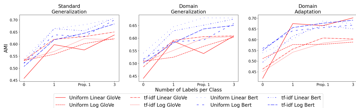
Figure 4: Average AMI performance for SGD Real (Standard Generalization, Domain Generalization, and Domain Adaptation) on three highly constrained few-shot settings: 1 shot, proportional 1 shot, and 3 shot.
