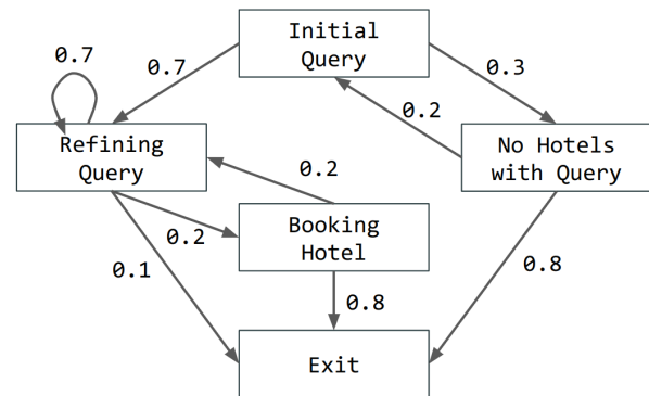
Figure 1: Example dialog structure for the goal-oriented task booking a hotel.
