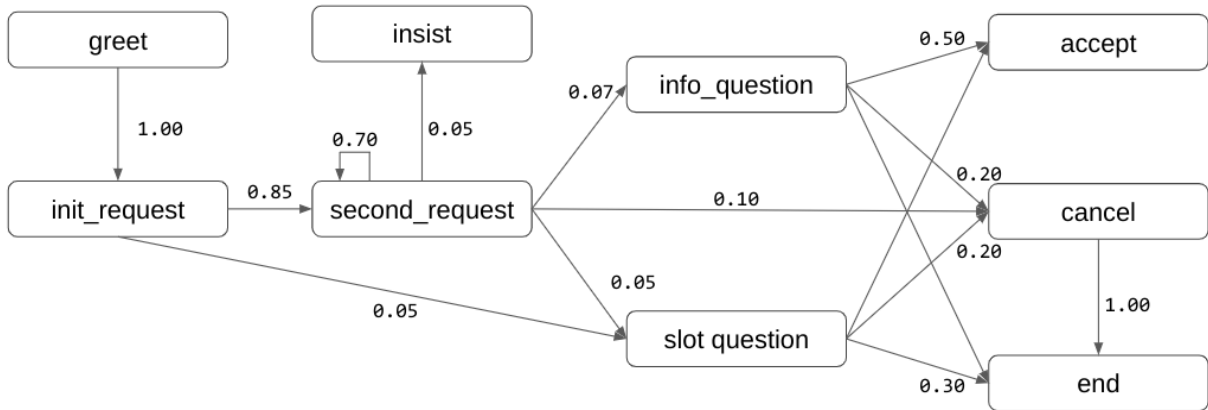
Figure 7: Ground truth dialog structure used to generate the MultiWoZ 2.1 dataset. The transition graph shows transitions over 0.05%.
