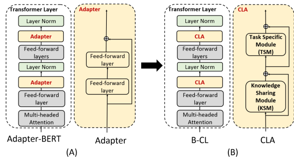
Figure 1: (A). Adapter-BERT (Houlsby et al., 2019) and its adapters in a transformer (Vaswani et al., 2017) layer. An adapter is a 2-layer fully connected network with a skip-connection. It is added twice to each Transformer layer. Only the adapters (yellow boxes) and layer norm (green boxes) layers are trainable. The other modules (grey boxes) are frozen. (B). Proposed B-CL, which replaces the adapter with CLA. CLA has two sub-modules: knowledge sharing module (KSM) and task specific module (TSM). Each of these modules has a skip-connection.
