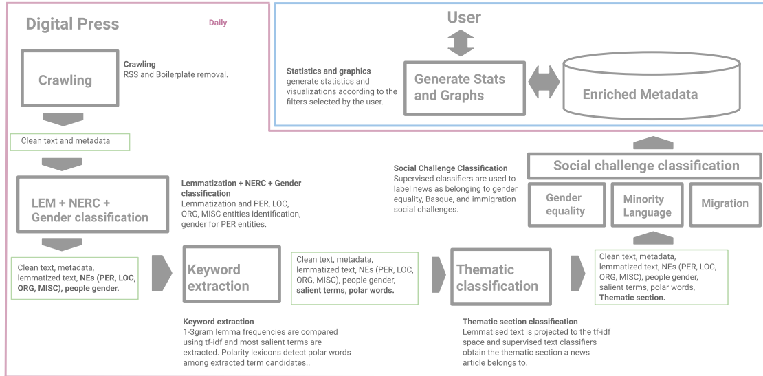
Figure 1: Architecture of GEPSA tool.
