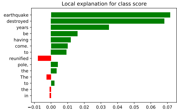
Figure 2: Explanations provided by the LIME Text Explainer (Ribeiro et al., 2016) on our example sentence. As the source sentence is fixed, we are only interested in the explanation of the target sentence. Each word can be seen as an interpretable feature holding a score that denotes its influence on the decision of the estimator.
