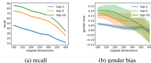
Figure 4: Effect of the number of clipped dimensions m on performance of recall and bias on MS-COCO 1K.
