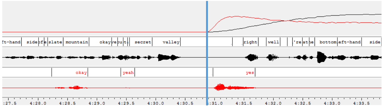
Example 1: Prediction in a pause. The model predicts that the red speaker will give a (short) response, but also that the black speaker will continue later on.
