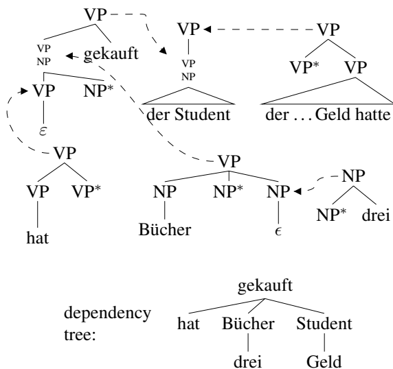
Figure 7: Derivation for (4)
