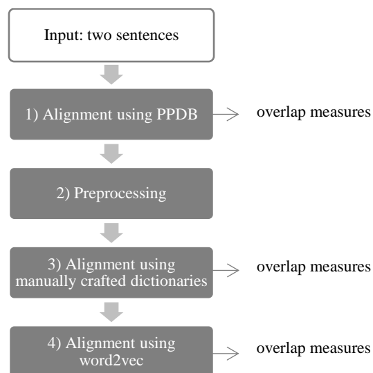
Figure 1: Aligning steps performed by the system
