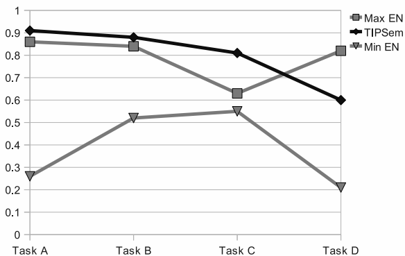
Figure 5: Spanish F_{\beta=1} indirect assessment
