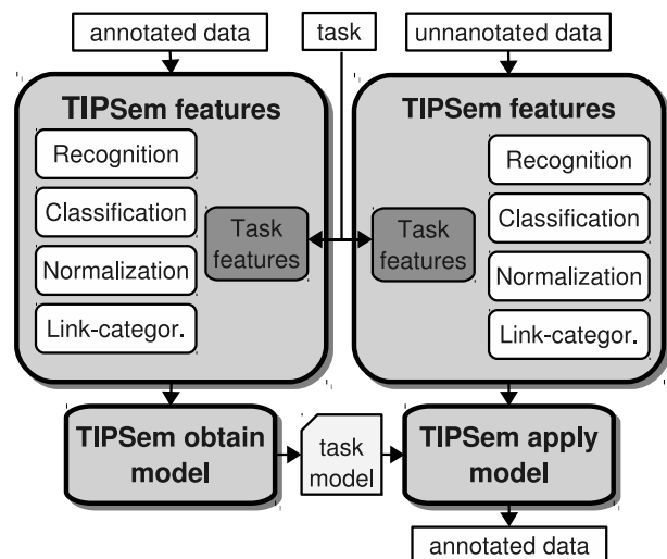
Figure 3: TIPSem architecture
