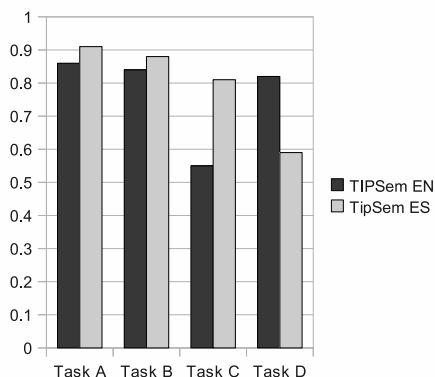
Figure 6: TIPSem EN - ES F_{\beta=1} comparative
