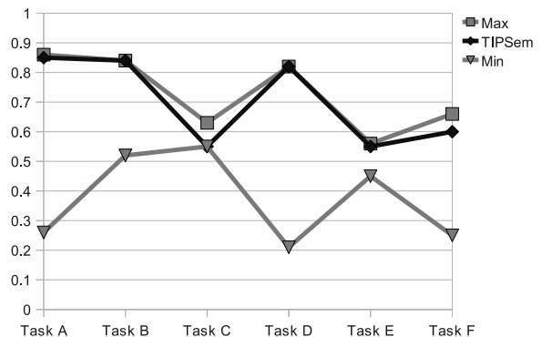
Figure 4: English F_{\beta=1} comparative
