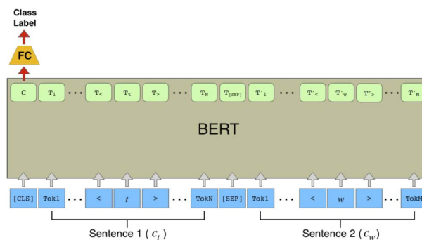
Figure 4: The contextual hypernym prediction model is based on BERT (Devlin et al., 2019). Input sentences c_t and c_w are tokenized, prepended with a [CLS] token, and separated by a [SEP] token. The target word t in the first sentence, c_t , and the related word w in the second sentence, c_w , are surrounded by < and > tokens. The class label ( hypernym or not ) is predicted by feeding the output representation of the [CLS] token through fully-connected and softmax layers.
