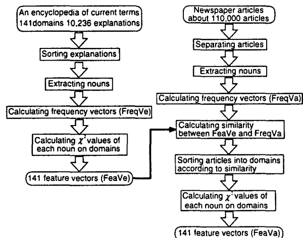
Figure 2: Calculating feature vectors
