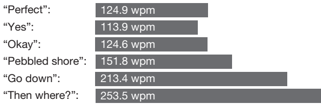
Figure 3: Mdn wpm for the six samples — TTS output
