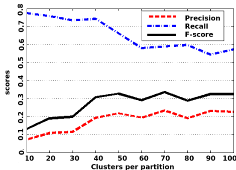
Figure 1: Variation in precision, recall and F-score on increasing the number of clusters per partition for the FSD dataset.
