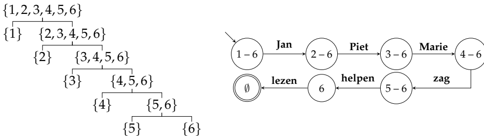
Figure 13 A right-branching recursive partitioning and an FA.
