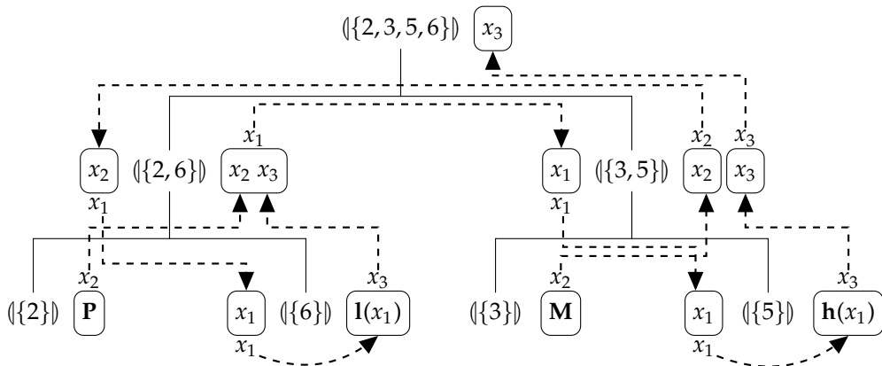
Figure 18 Derivation tree for the recursive partitioning of Figure 17, induced by the sDCP rules.
