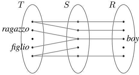
Figure 1: Relationships between Source, Target and Resource Vocabularies.
