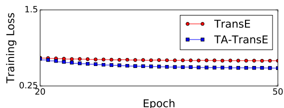
Figure 3: Training loss in YAGO15K. TA-TRANSE’s ability to learn from time information leads to a lower loss.
