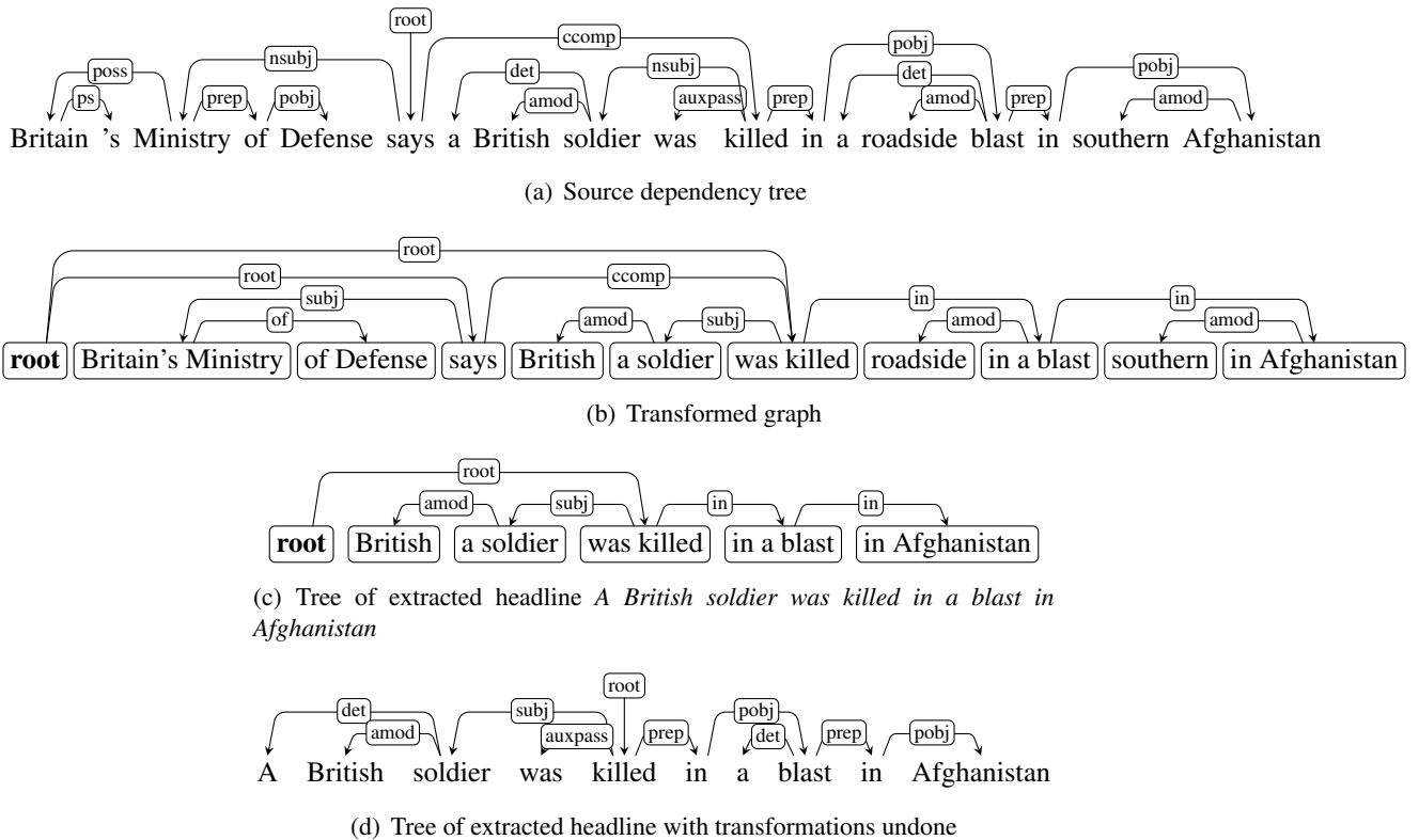
Figure 1: Source, transformed and extracted trees given headline British soldier killed in Afghanistan
