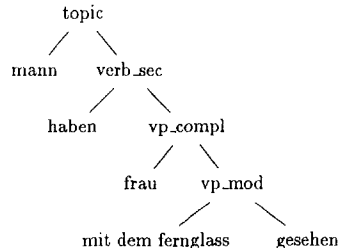
Figure 3: Derivation tree of German example
