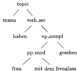
Figure 4: Derivation tree of alternative reading
