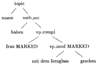
Figure 5: Marked tree of German example
