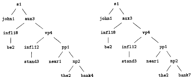
Figure 1: Derivation trees
