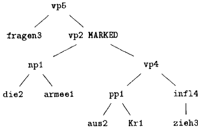
Figure 2: Marked derivation tree
