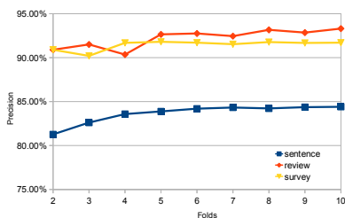
Figure 1: Sentiment classification accuracy using variable cross-validation
