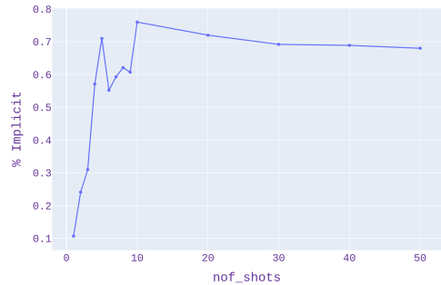
Figure 3: (nof_shots) x (% Implicit) line curve. Optimal number of shots for the best generator OPG: (1)+(2)+(3)+(4).
