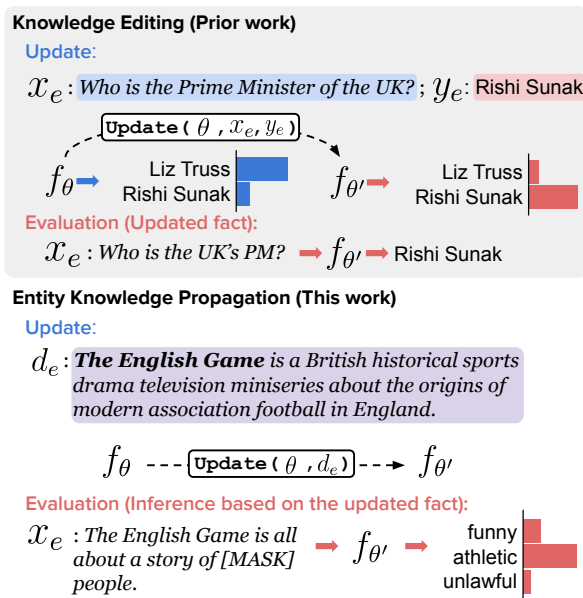
Figure 1: Knowledge editing tasks. We study a challenging entity knowledge propagation task where language models should make inferences after learning entities from their definitions. This differs from past knowledge editing which evaluates paraphrases of injected facts.
