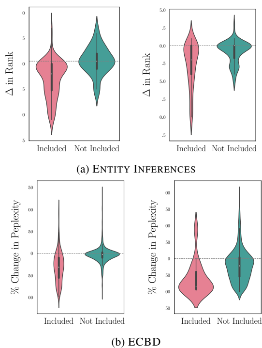
Figure 3: (Left) Fine-tuning performance on GPT-Neo split by whether the gold span is included in the definition sentence or not. (Right) Input augmentation performance on GPT-Neo split by whether the gold span is included in the definition sentence or not.
