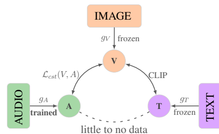
Figure 3: Learning paradigm of vIP \sim \mathcal{A}_N \mathcal{T} .
