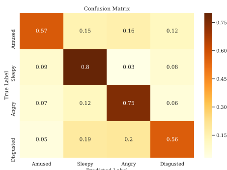
Figure 8: Seq2Seq-EVC
