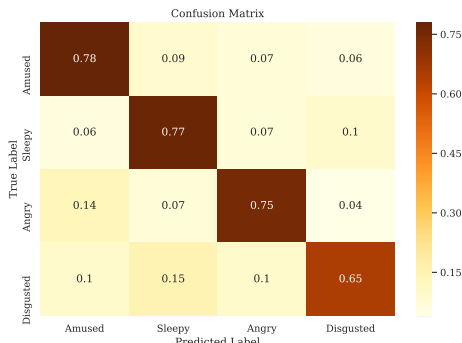
Figure 7: Ours -
