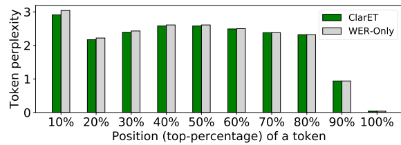
Figure 7: Token-level perplexity w.r.t tokens’ percentage positions in events on held-out dev set.
