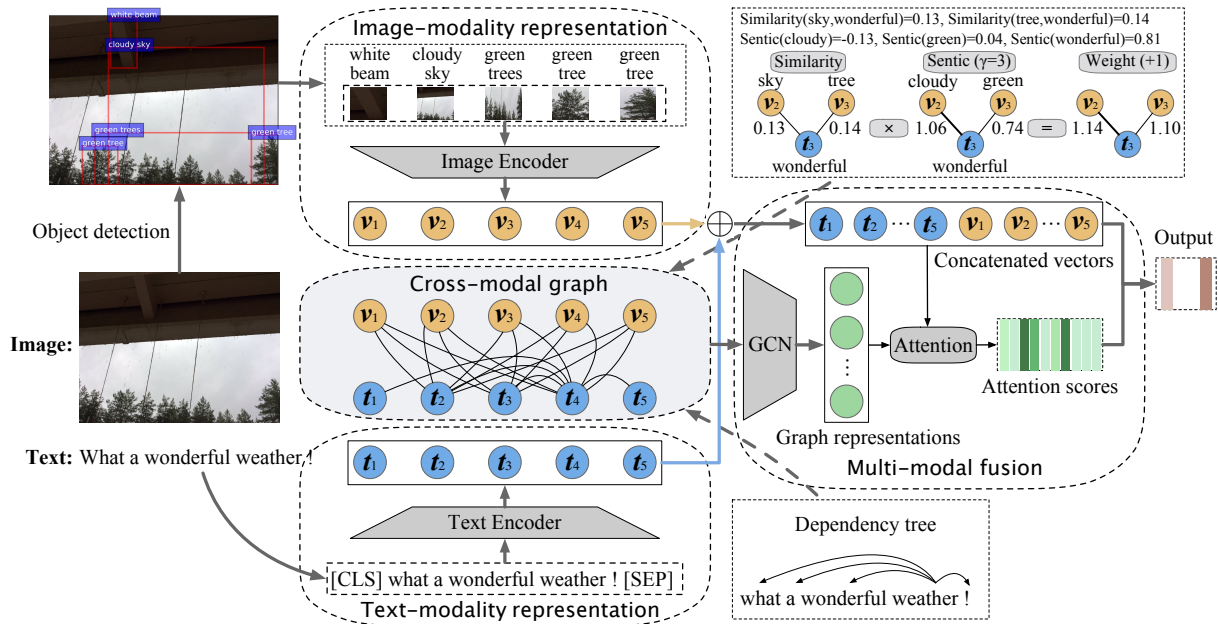
Figure 2: The architecture of the proposed CMGCN. \oplus represents matrix concatenation.
