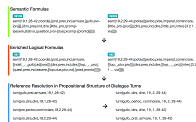
Figure 4: Excerpt of DU n.19 showing only the semantic and pragmatic conversion steps.
