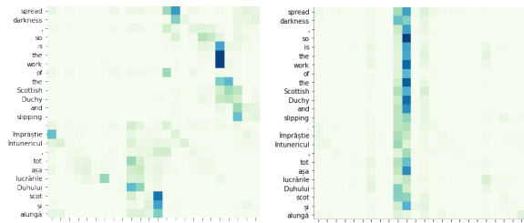
Figure 3: Example of two attention maps from particular heads that perform well on source AUC (left) and target AUC (right) for RO-EN.
