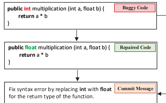
Figure 1: An illustrative example for our proposed task. Given a buggy code, the task is to generate its corresponding repaired version, as well as the commit message that describes their changes.
