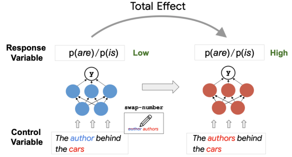
Figure 2: Total effects are measured by performing an intervention on the prompt (here, changing the grammatical number of the main subject), and measuring the relative change in the response variable (the ratio of probabilities of the originally incorrect verb form over the originally correct verb form).
