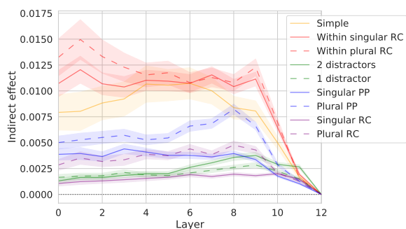
Figure 9: Natural indirect effects of the top 5% of neurons in each layer of XLNet.
