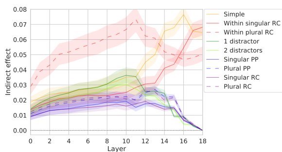
Figure 8: Natural indirect effects of the top 5% of neurons in each layer of Transformer-XL.
