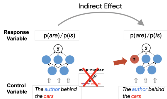
Figure 5: Indirect effects are measured by setting an individual neuron to the value it would have taken had the intervention occurred, then measuring the relative change in the response variable.
