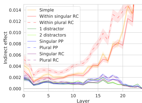
Figure 7: Natural indirect effects of the top 5% of neurons in each layer of GPT-2 Medium.
