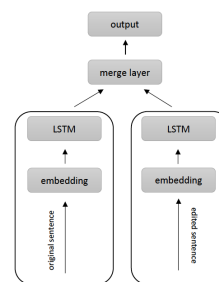
Figure 1: Twin LSTM
