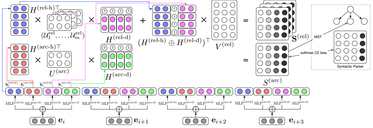
Figure 8: The overview of our transformer-based biaffine dependency parsing model.
