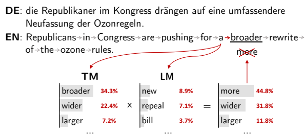
Figure 4: Example of failure of probability interpolation between LM and TM, while translating DE→EN.
