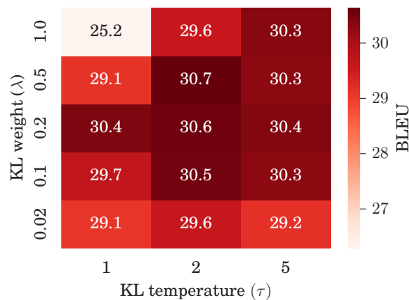
Figure 5: BLEU scores on the DE-EN dev set of models trained with different \lambda and \tau for the \mathcal{L}_{KL} . Mean of 3 runs for each combination reported.
