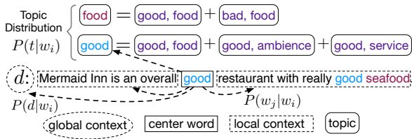
Figure 3: Embedding training.
