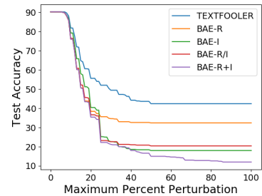
(a) Word-LSTM
