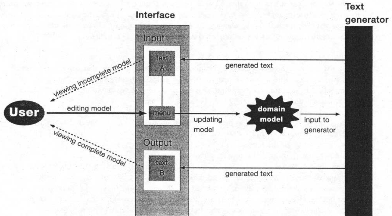
Figure 2: The WYSIWYM architecture
