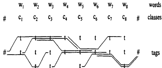
Figure 3: Incompatible sequences in the tag space of a sentence
