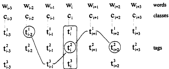
Figure 1: Disambiguation of classes between two selected tags
