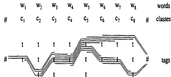
Figure 2: Two valid paths through the tag space of a sentence
